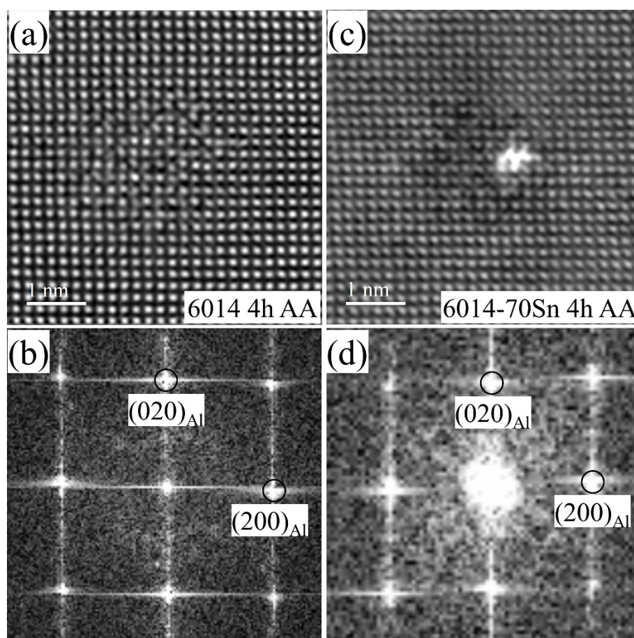
Fig. S1. HAADF-STEM image of PA cluster formed after 4 h ageing at 180 °C in the alloy (a) 6014, (c) 6014-70Sn. (b, d) corresponding fast Fourier transform patterns of (a, c), respectively.
